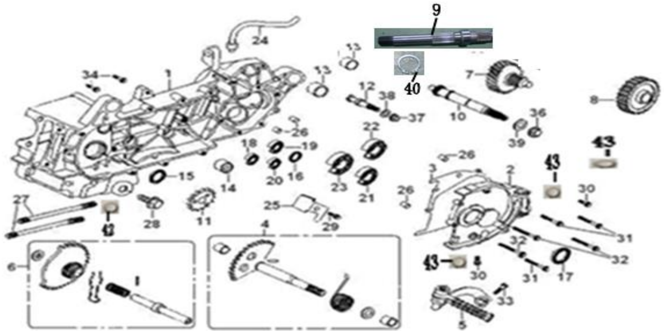
FIG 5 - LEFT CRANK CASE Cont'd
