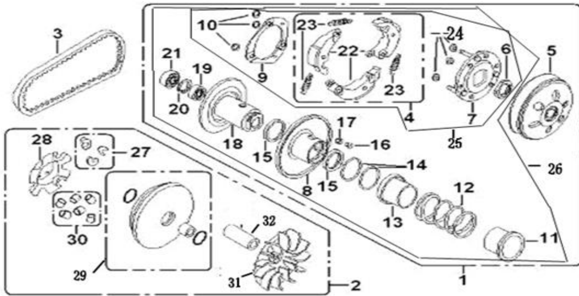
FIG 9 - VARIATOR AND CLUTCH
