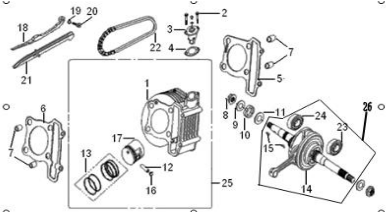
FIG 2 - CYLINDER Cont'd
