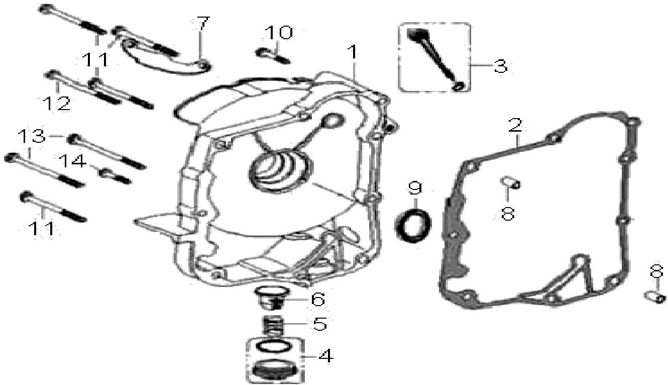
FIG 6 - RIGHT OIL COVER
