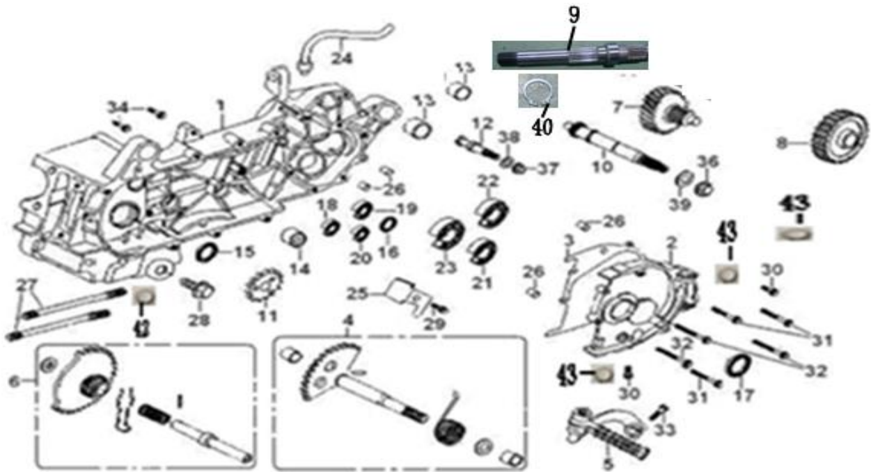
FIG 5 - LEFT CRANK CASE Cont'd
