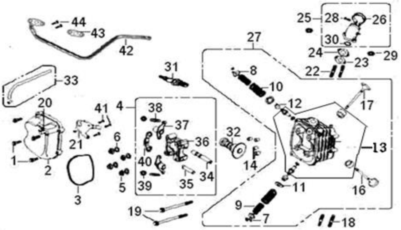
FIG 3 - CYLINDER HEAD Cont'd
