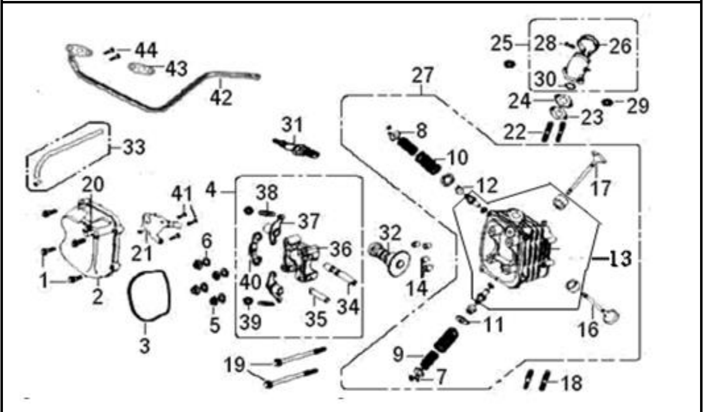
FIG 3 - CYLINDER HEAD - Cont'd
