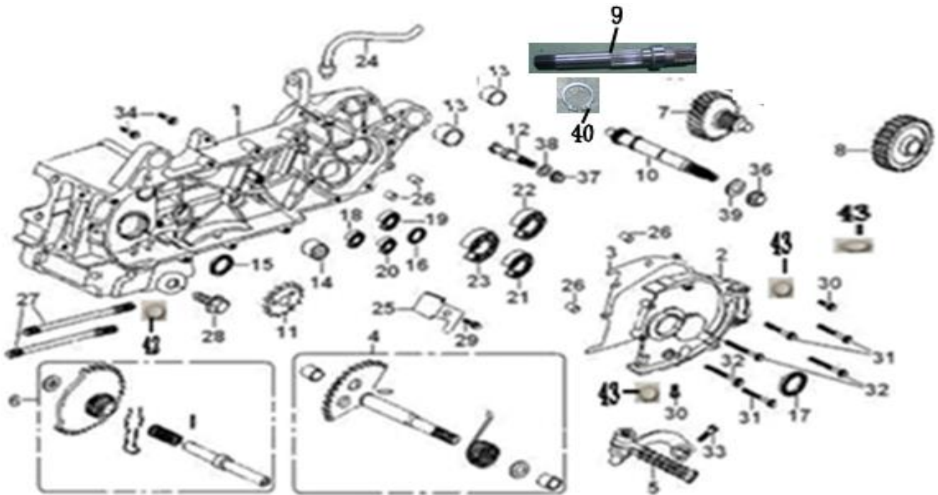
FIG 5 - LEFT CRANK CASE
