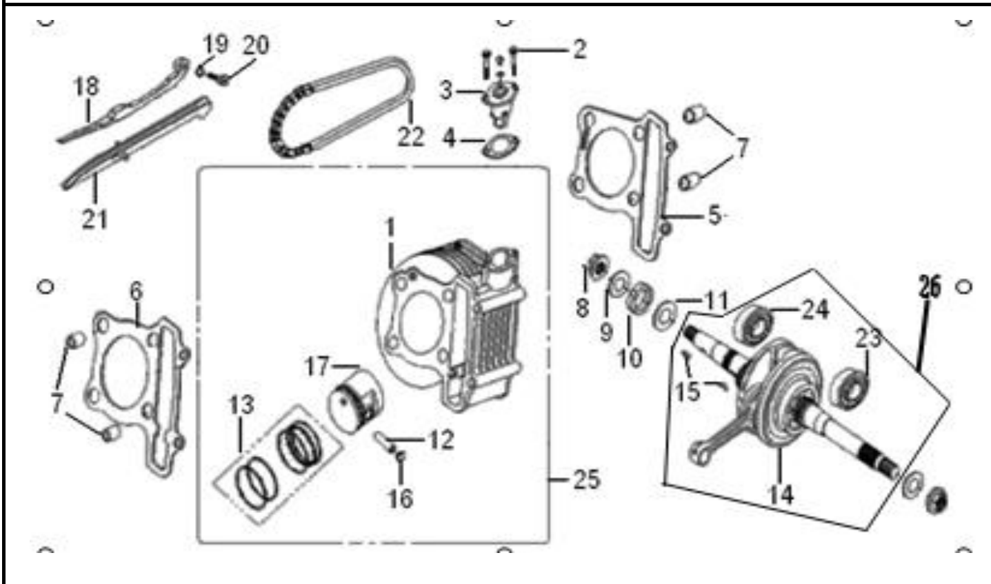
FIG 2 - CYLINDER
