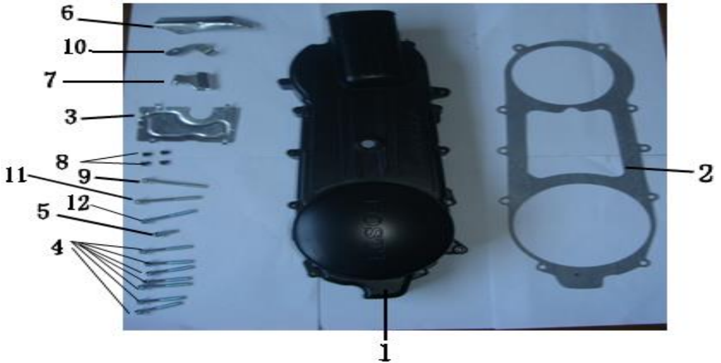
FIG 7 - RIGHT CRANKCASE COVER
