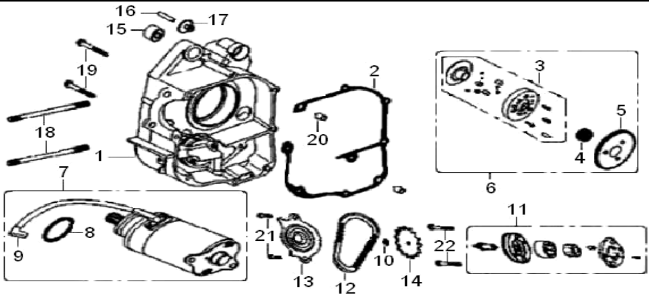
FIG 4 - RIGHT SIDE CRANK CASE
