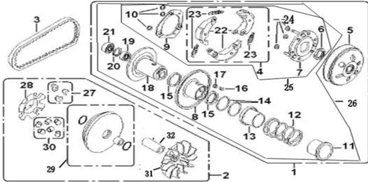
FIG 9 - VARIATOR AND CLUTCH Cont'd
