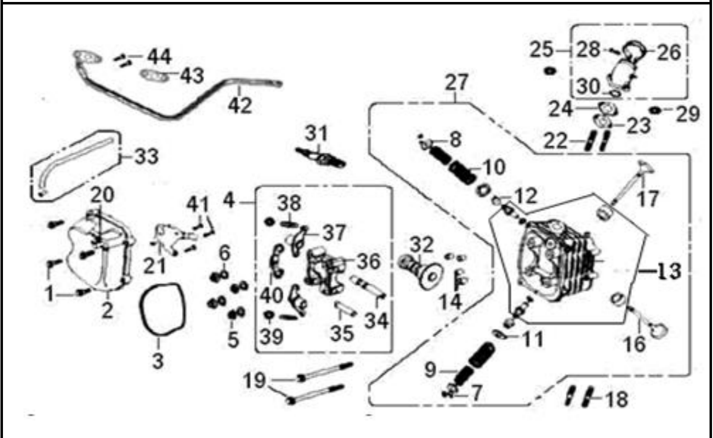
FIG 3 - CYLINDER HEAD
