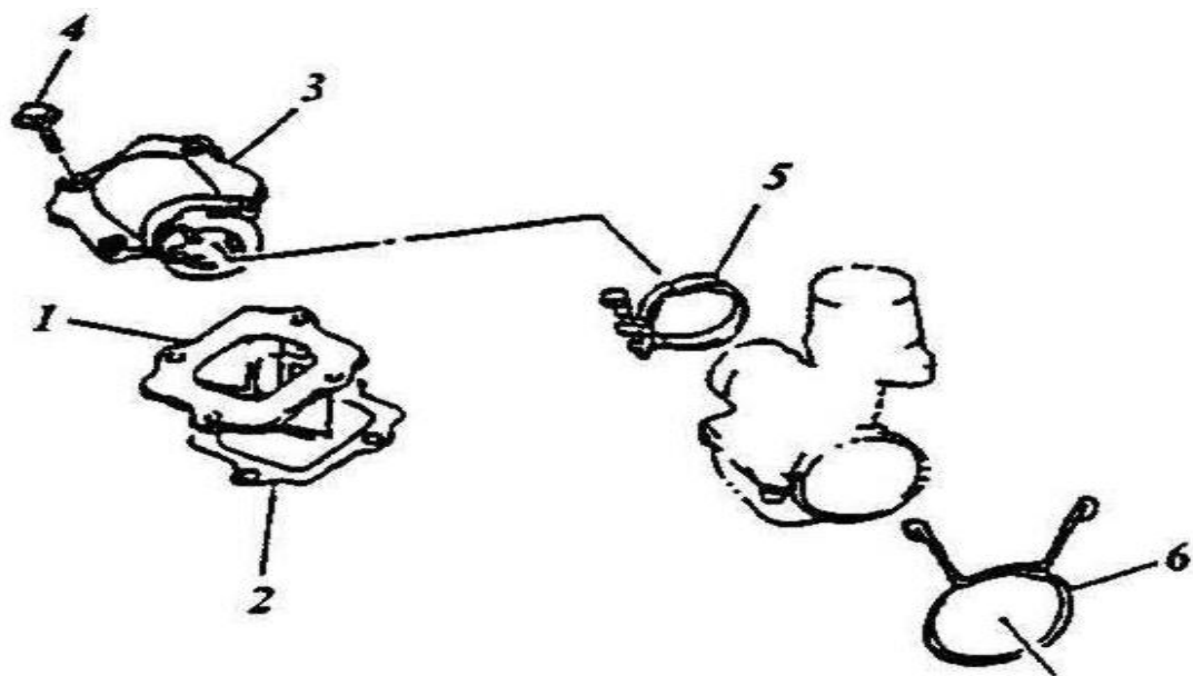
116-E05 REED VALVE, AIR CLEANER
