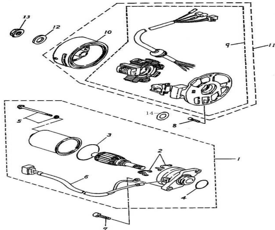
116-E07 GENERATOR, STARTING MOTOR
