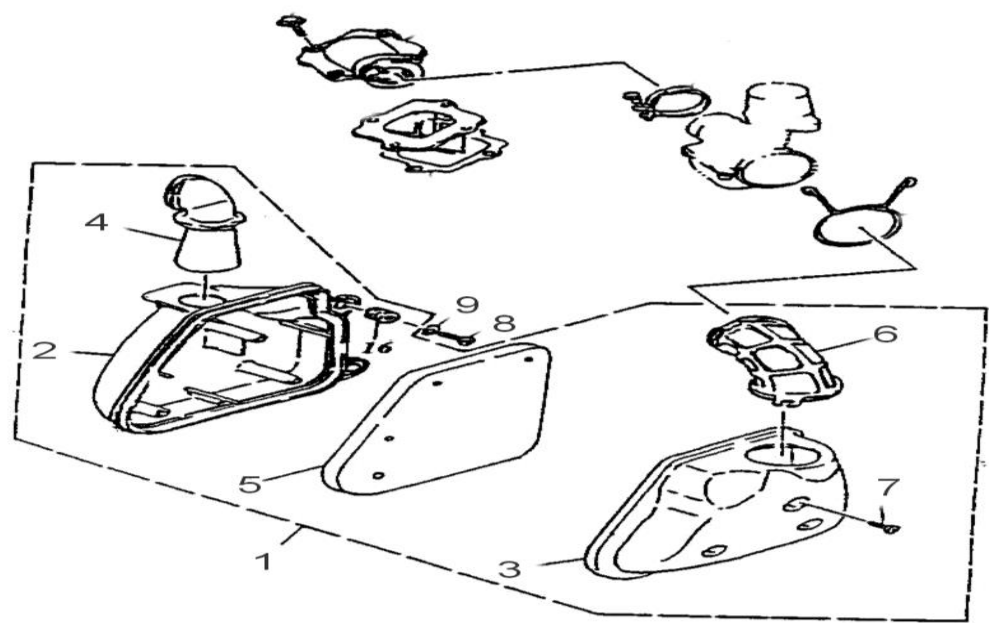
116-F01 AIR CLEANER
