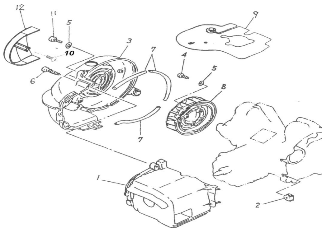
116-E03 FAN, AIR SHROUD
